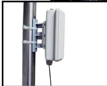
Vertical mast
